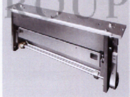
HARD METAL VERTICAL BLADE CARTRIDGE TC 7530 (strip cut 5/16")
